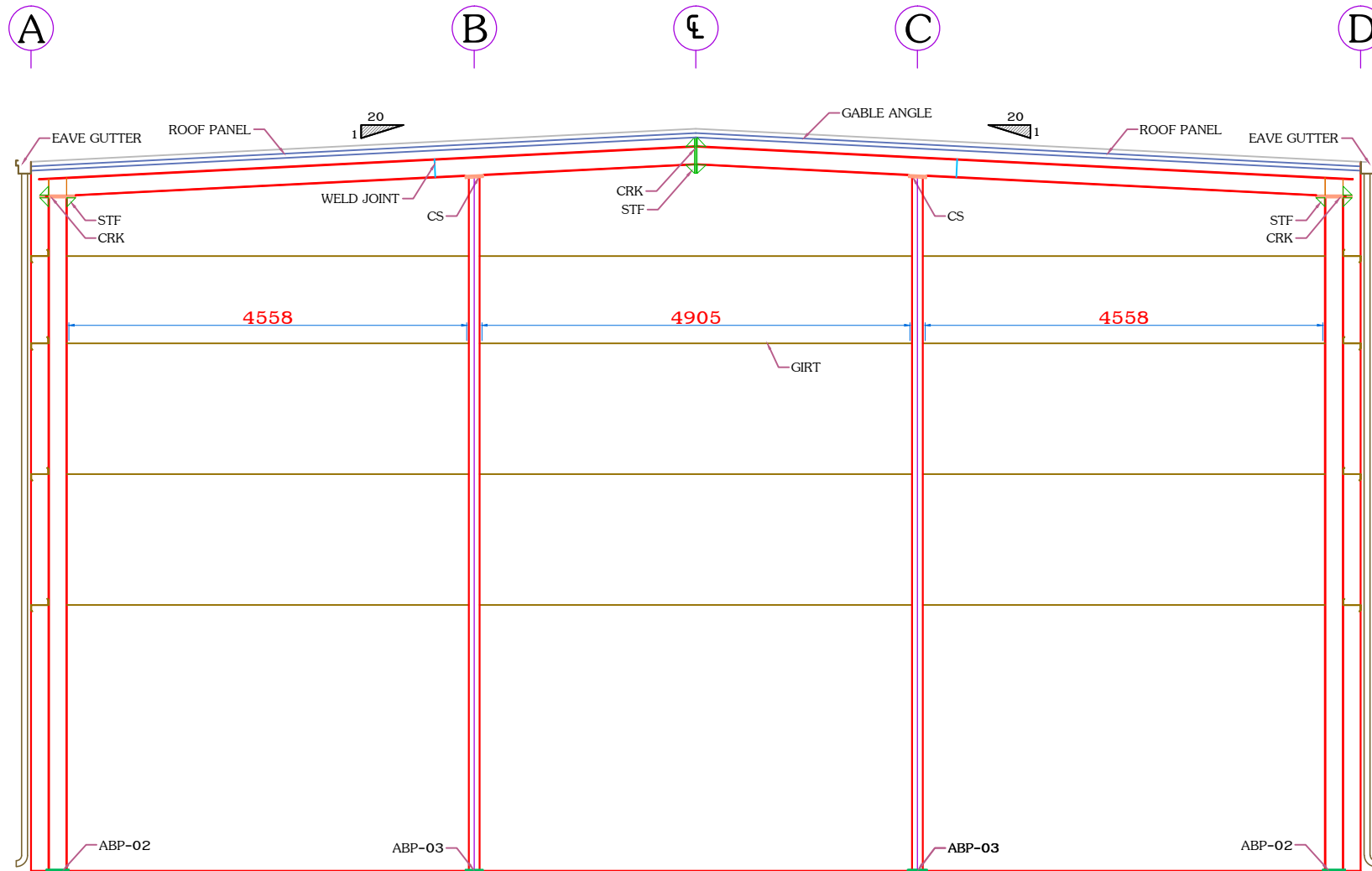
END WALL FRAMING @ GRID-1
